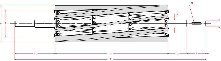
Rulli Master Aperti / Open Master Rolls
