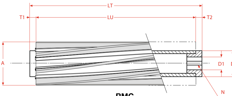
Rulli Master Chiusi/ Closed Master Rolls
